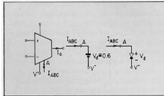
Fig. 11 Macromodel of bias current port on bipolar OTA.
