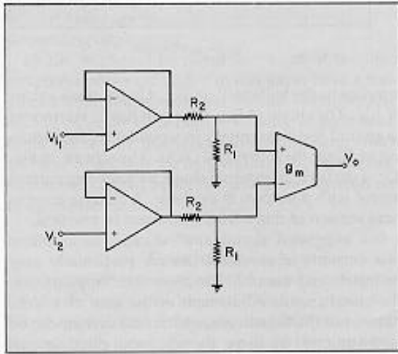
Fig. 10 Signal conditioner for OTAs.
