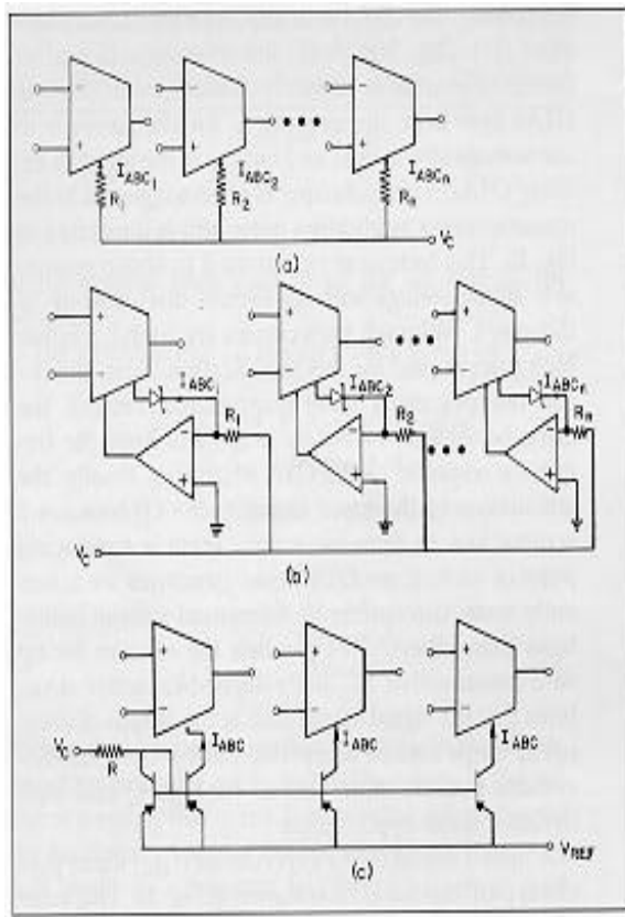
Fig. 13 Schemes for simultaneous g_m adjustment.
